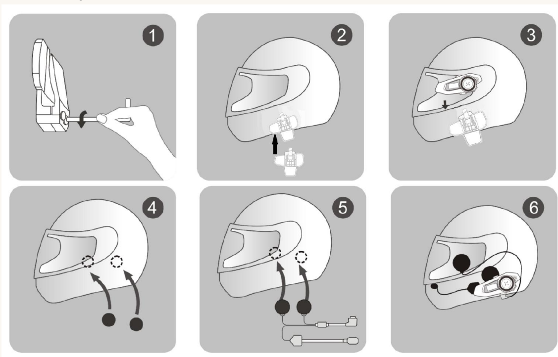
Clamp mounting, steps 1–6
